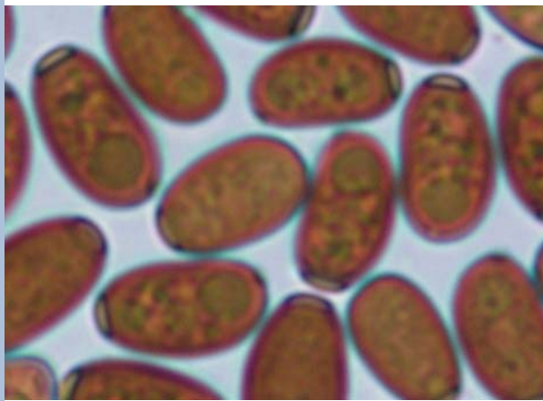
prominenter Keimporus Sporen
